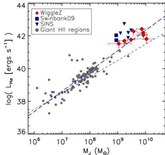
Figure 12: Scaling of H \alpha luminosity (proxy for star-formation rate) with inferred clump Jeans mass M_J = \pi^2 r \sigma^2 / 6G from local HII regions up to the most luminous z > 1 clumps. The correlation is quite tight and the slope close to unity (black dashed line). The blue dashed line is the best fit slope M_J^{1.24} . Credit: reproduced from Figure 5 of Wisnioski et al. (2012).
