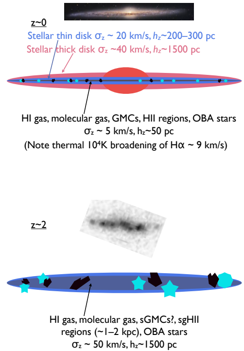
Figure 2: Illustrative schematic showing the different structures of low-redshift and high-redshift disc galaxies in an edge-on view. Top: components of the Milky Way and similar local spirals (see Section 1.2.2) containing stellar thin/thick discs and a very thin gas disc in the centre. The latter contains all the Giant Molecular Clouds, HII regions, molecular and neutral gas and young stars. Bottom: a clumpy high-redshift disc (see Section 5.1). This contains a thick ( \sim 1\text{ kpc} scaleheight) and highly turbulent discs of molecular gas, young stars, super-giant HII regions (kpc scale star-forming ‘clumps’) and (presumably) super-Giant Molecular Clouds. Credit: inset images are of NGC 4565 (top, reproduced by permission of R. Jay Gabany, Cosmotography.com) and z \sim 3 galaxy UDF #6478 of Elmegreen & Elmegreen (2006) (their Figure 2, reproduced by permission of the AAS).
